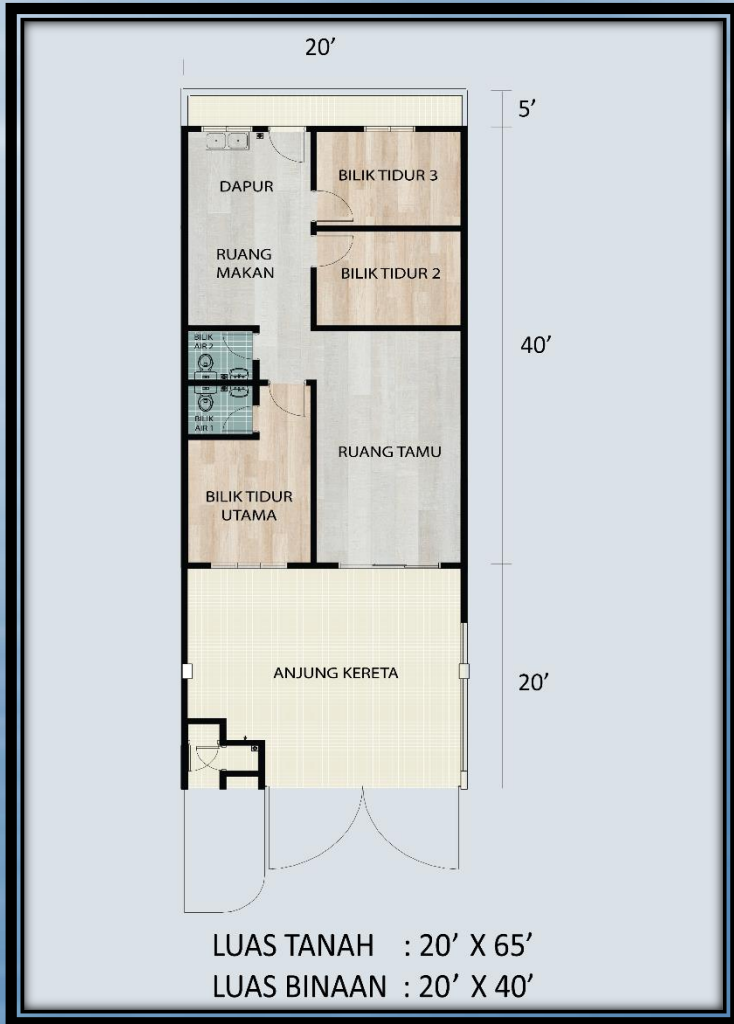
Single Storey Terrace House
